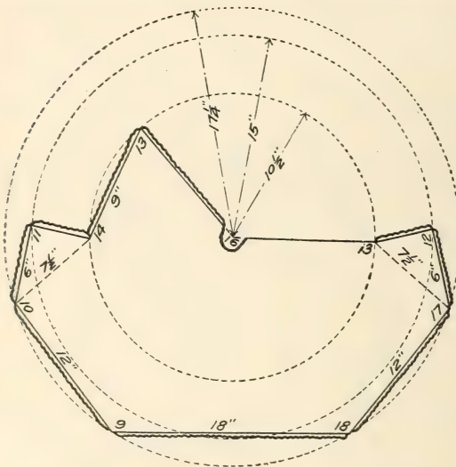
FIG. 5.—Pattern for second funnel of trap shown in Figure 2.
